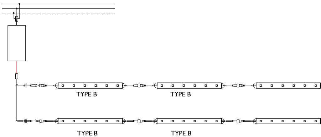
4, Series + Parallel connection Max 12pcs (150W)
