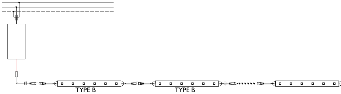
3, Series connection of up to 10pcs
