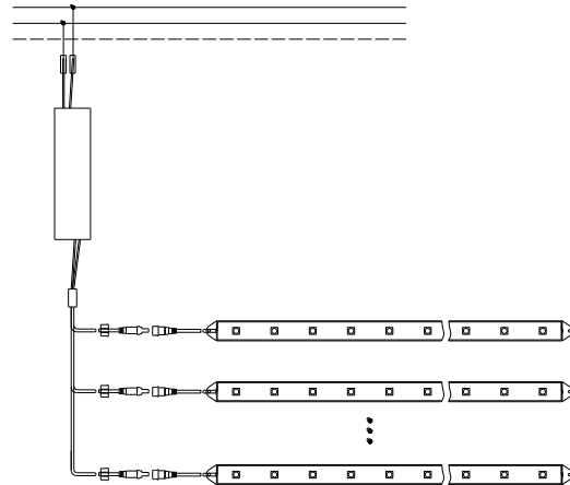
2, Parallel connection of up to 12pcs (150W)
